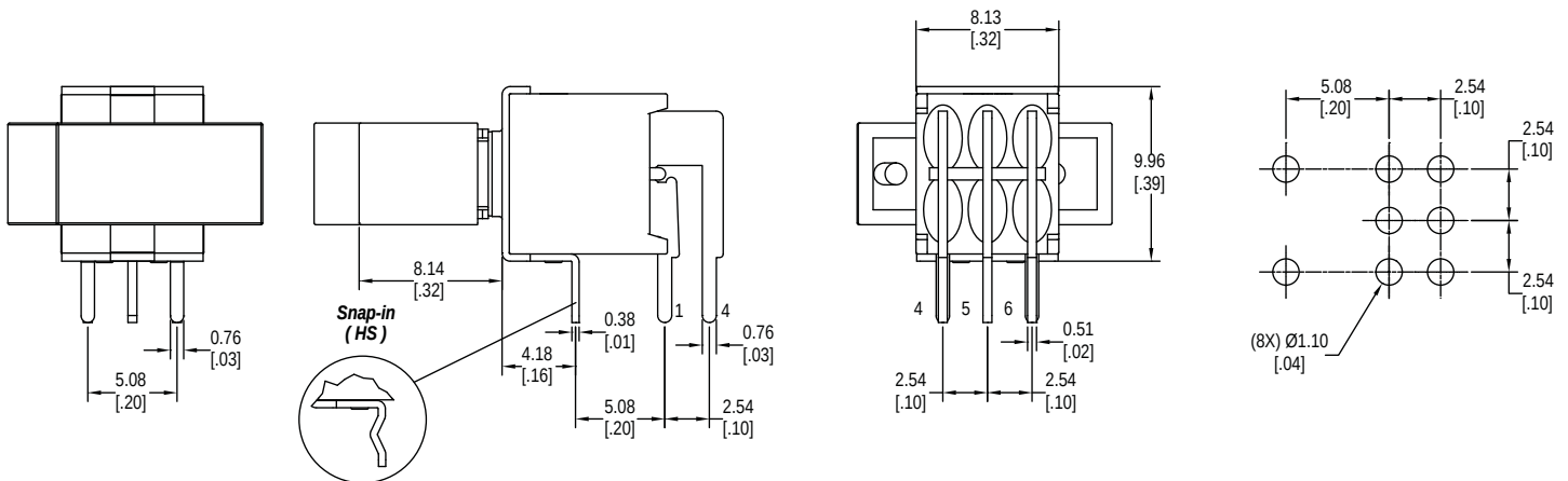
H (HS - Snap In) = Horizontal mount, right angle PC pins, double pole
